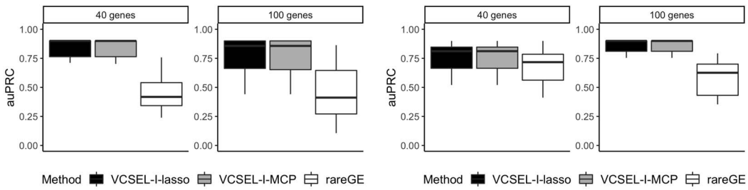
FIG. 2. The auPRCs of VCSEL-I-lasso, VCSEL-I-MCP, and rareGE under 40 and 100 genes for models with six nonzero variance components, using haplotype data from the SKAT R-package. True variance component values in the left panel mimic low LD scenario (14) while those in the right panel mimic high LD scenario (15).
